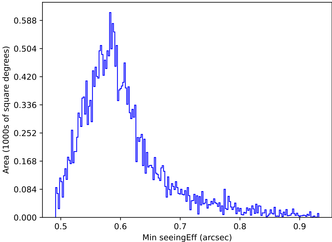
early_u_fpextra2.0_v3.4_10yrs All sky all bands: Min seeingEff
