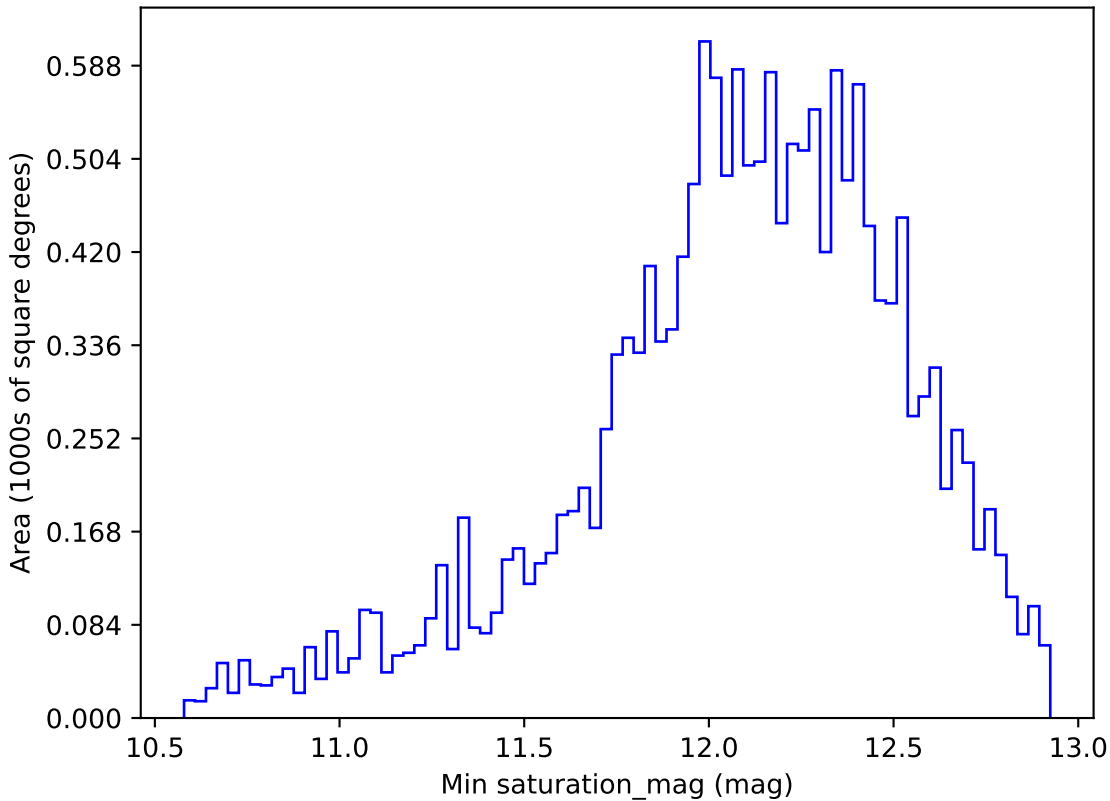
early_u_fpextra2.0_v3.4_10yrs WFD z band: Min saturation_mag
