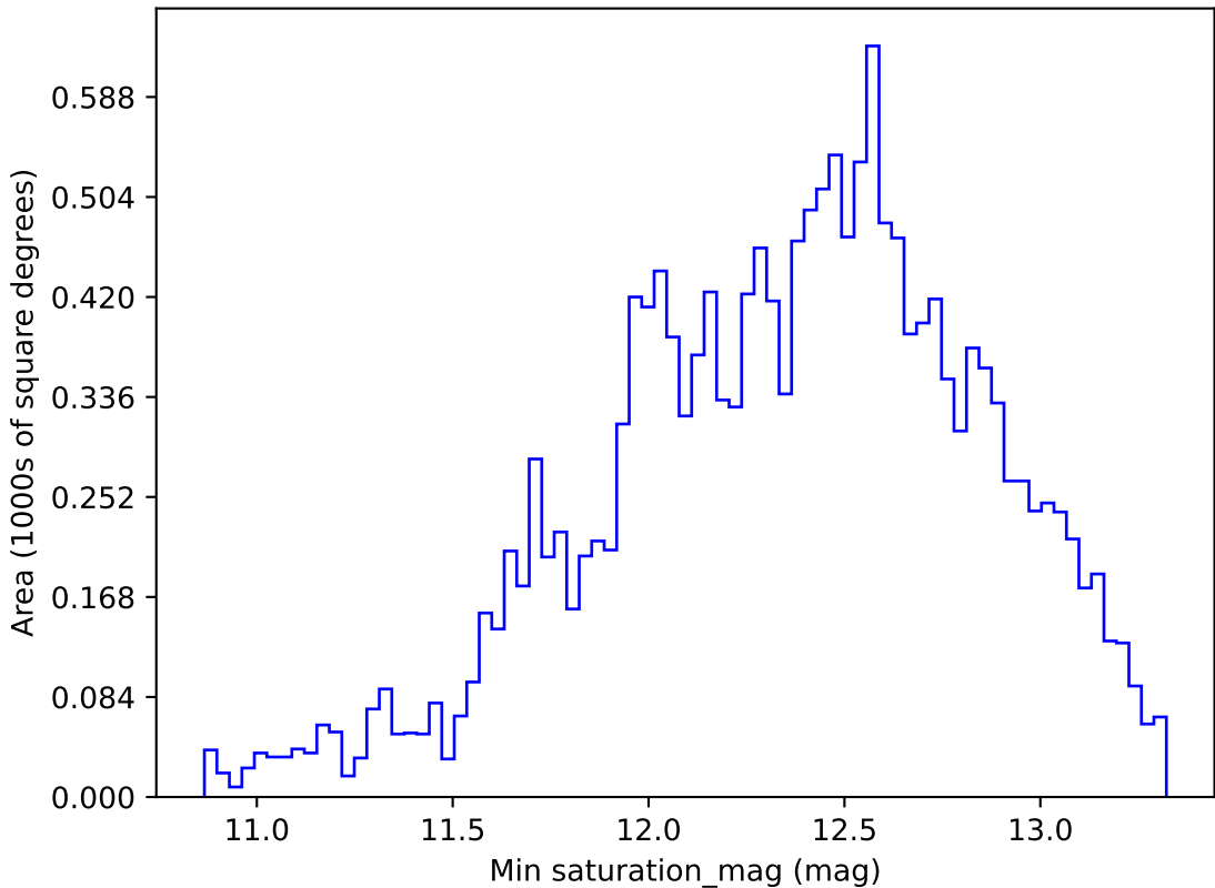
early_u_fpextra2.0_v3.4_10yrs WFD i band: Min saturation_mag
