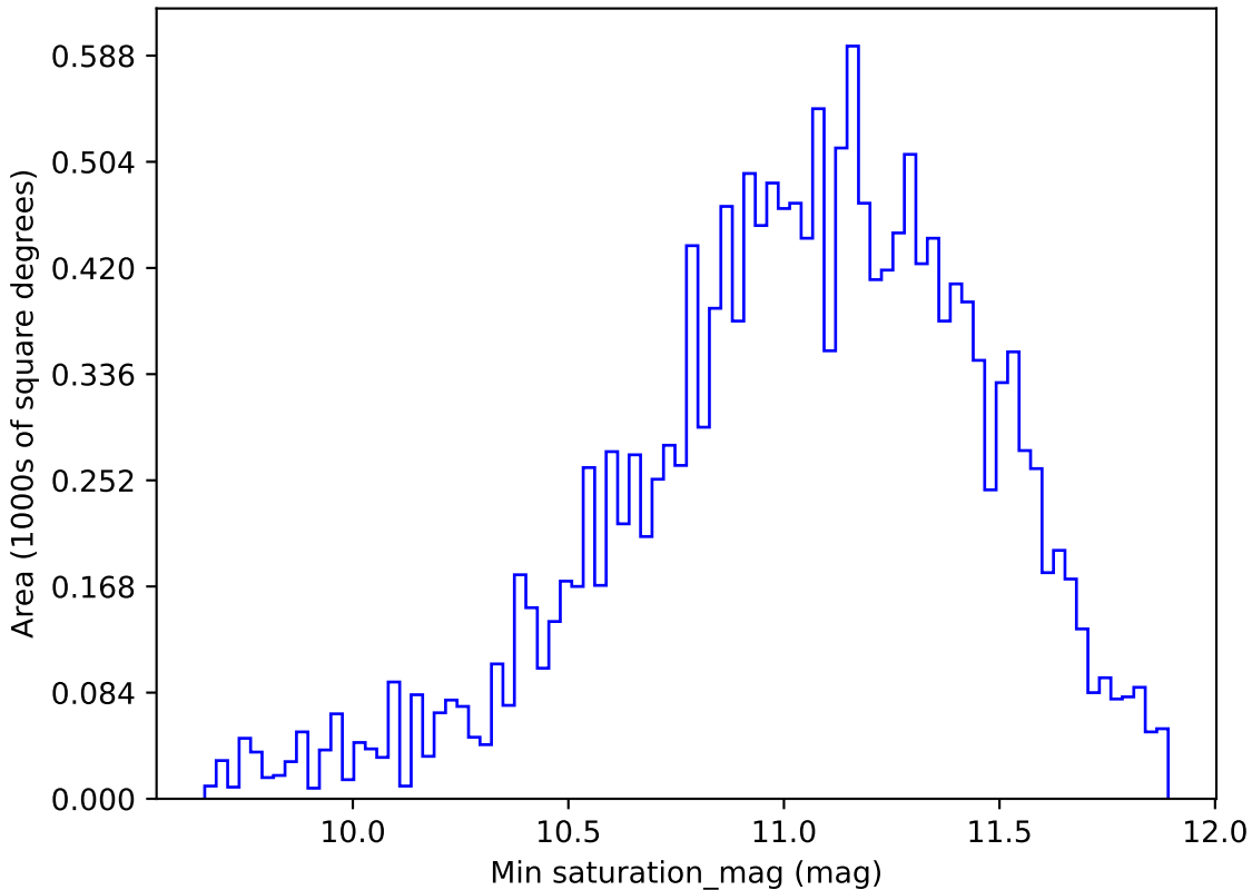
early_u_fpxtra2.0_v3.4_10yrs WFD all bands: Min saturation_mag
