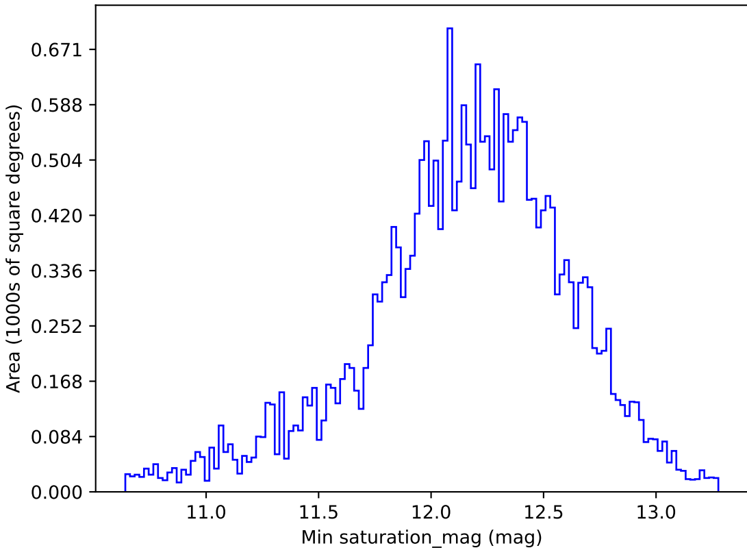
early_u_fpextra2.0_v3.4_10yrs All sky z band: Min saturation_mag
