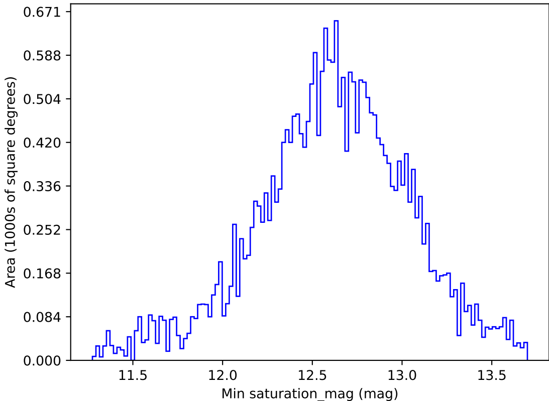
early_u_fpextra2.0_v3.4_10yrs All sky r band: Min saturation_mag
