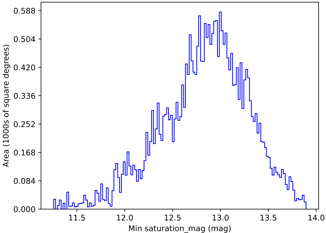
early_u_fpextra2.0_v3.4_10yrs All sky g band: Min saturation_mag
