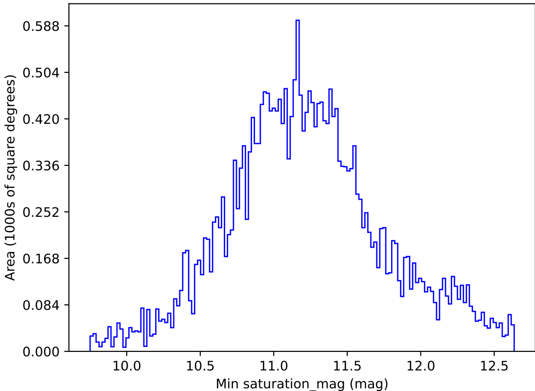
early_u_fpextra2.0_v3.4_10yrs All sky all bands: Min saturation_mag
