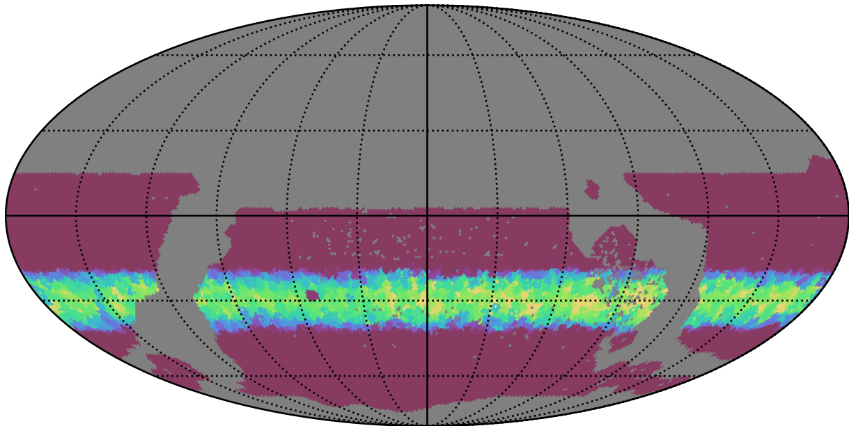
early_u_fpextra2.0_v3.4_10yrs WFD z band: Min normairmass
