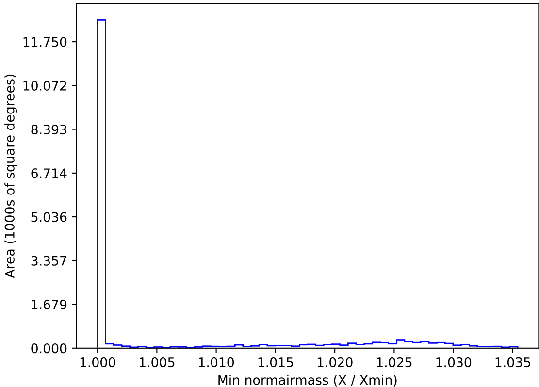
early_u_fpextra2.0_v3.4_10yrs WFD z band: Min normairmass
