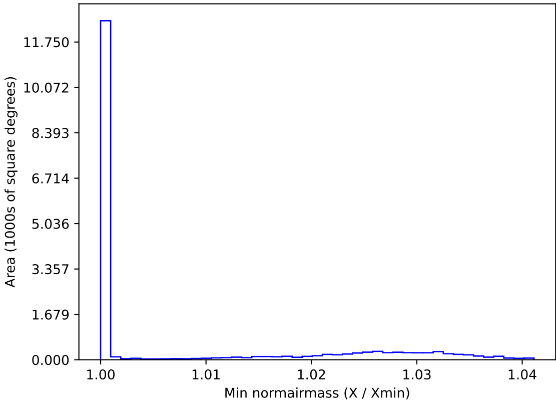
early_u_fpextra2.0_v3.4_10yrs WFD y band: Min normairmass
