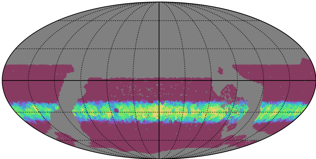
early_u_fpextra2.0_v3.4_10yrs WFD r band: Min normairmass
