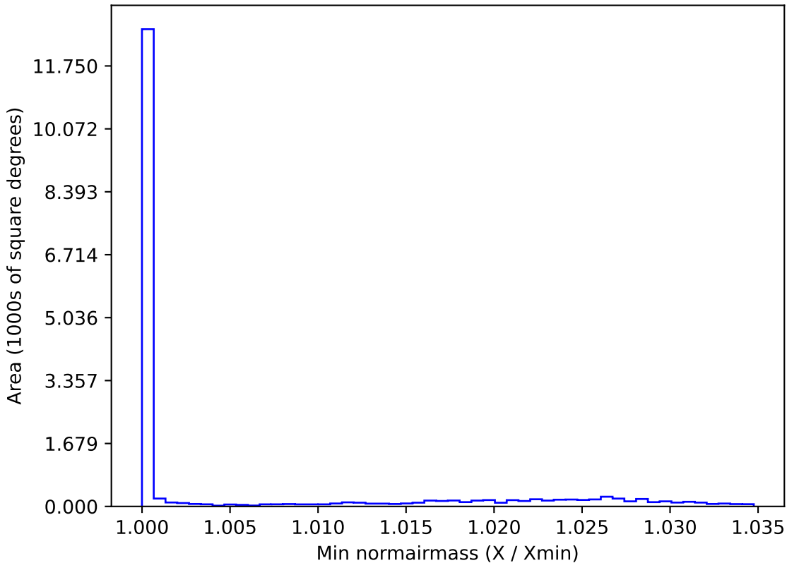
early_u_fpextra2.0_v3.4_10yrs WFD r band: Min normairmass
