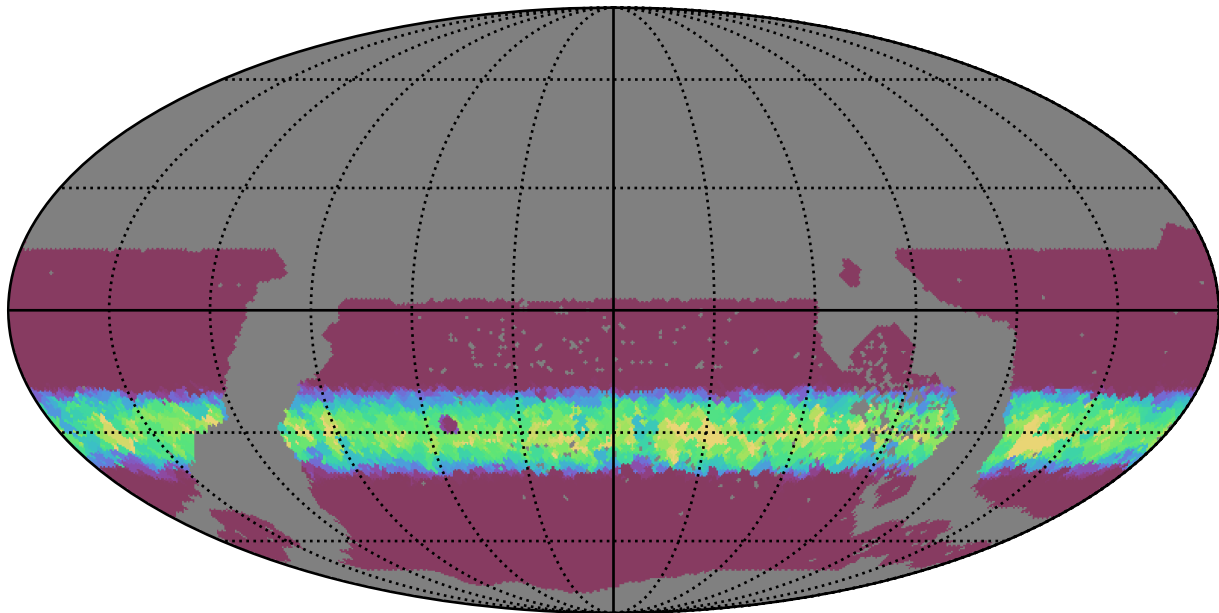
early_u_fpextra2.0_v3.4_10yrs WFD i band: Min normairmass
