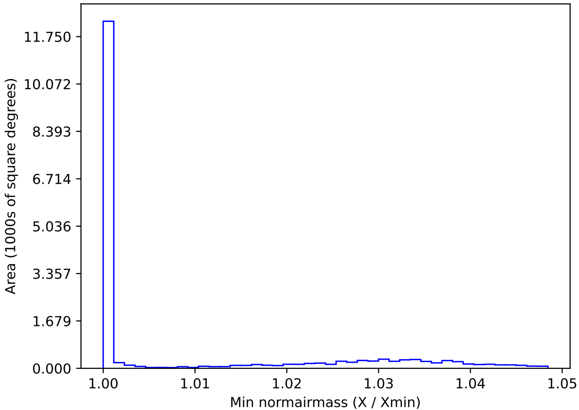
early_u_fpextra2.0_v3.4_10yrs WFD g band: Min normairmass
