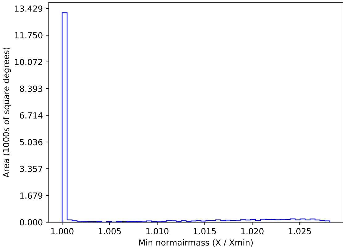
early_u_fpextra2.0_v3.4_10yrs WFD all bands: Min normairmass
