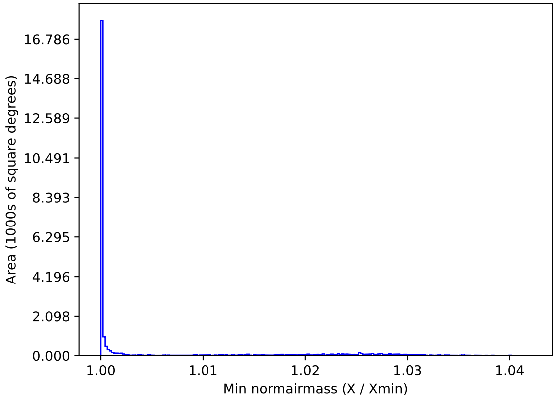
early_u_fpextra2.0_v3.4_10yrs All sky z band: Min normairmass
