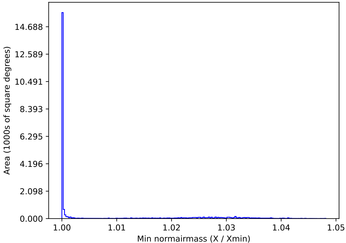
early_u_fpextra2.0_v3.4_10yrs All sky y band: Min normairmass
