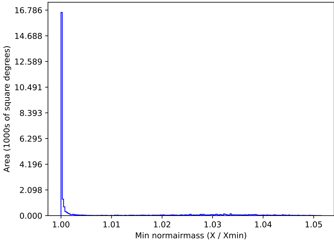
early_u_fpextra2.0_v3.4_10yrs All sky g band: Min normairmass
