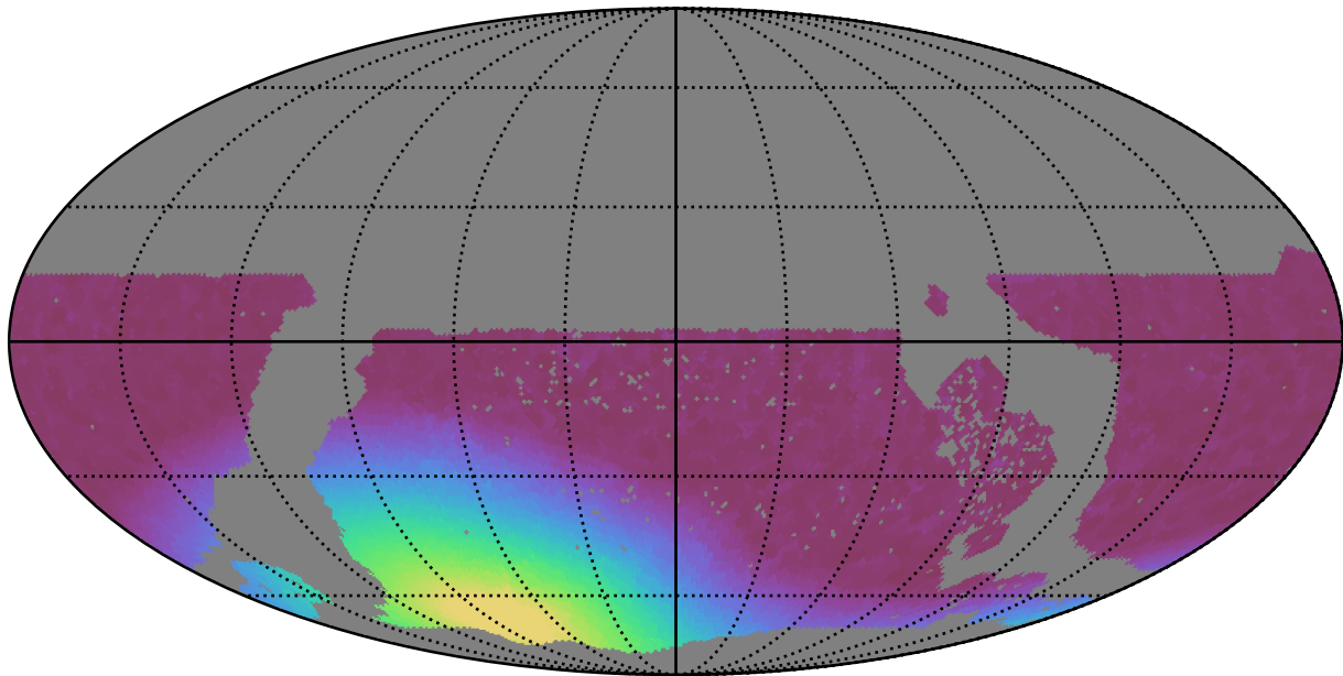
early_u_fpextra2.0_v3.4_10yrs WFD z band: Min moonDistance
