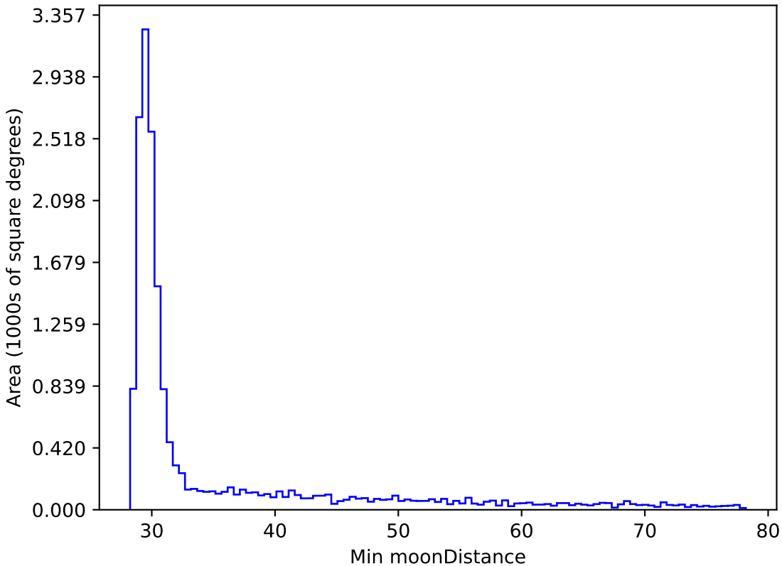
early_u_fpextra2.0_v3.4_10yrs WFD z band: Min moonDistance
