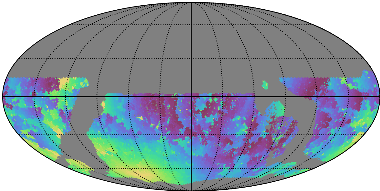
early_u_fpextra2.0_v3.4_10yrs WFD u band: Min moonDistance
