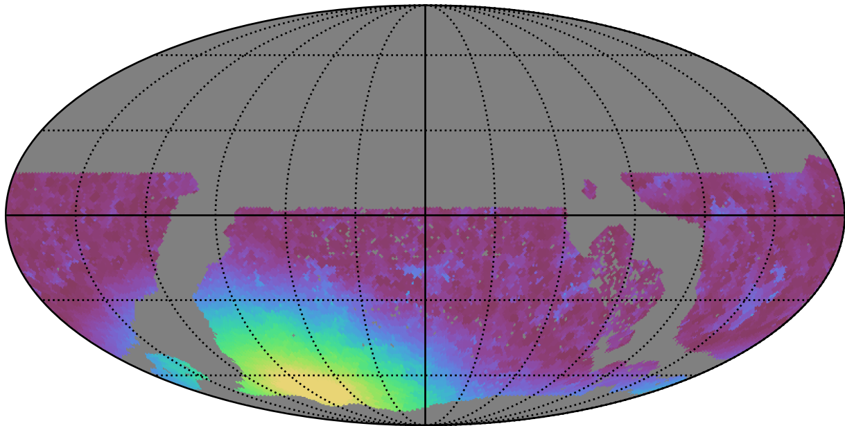
early_u_fpextra2.0_v3.4_10yrs WFD r band: Min moonDistance
