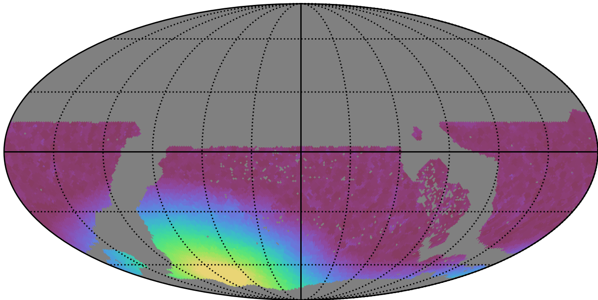
early_u_fpextra2.0_v3.4_10yrs WFD i band: Min moonDistance
