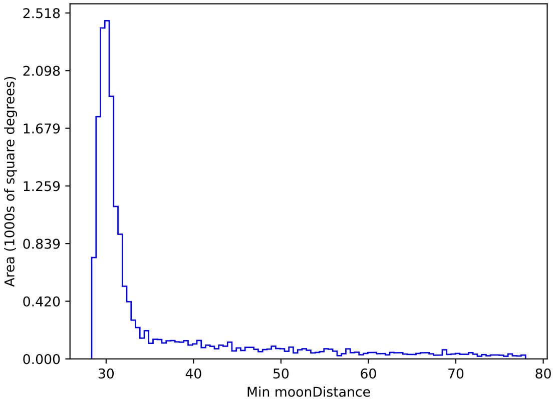
early_u_fpextra2.0_v3.4_10yrs WFD i band: Min moonDistance
