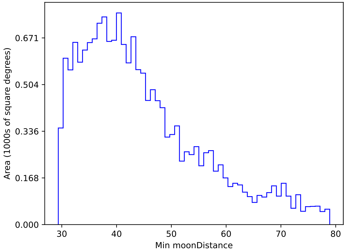
early_u_fpextra2.0_v3.4_10yrs WFD g band: Min moonDistance
