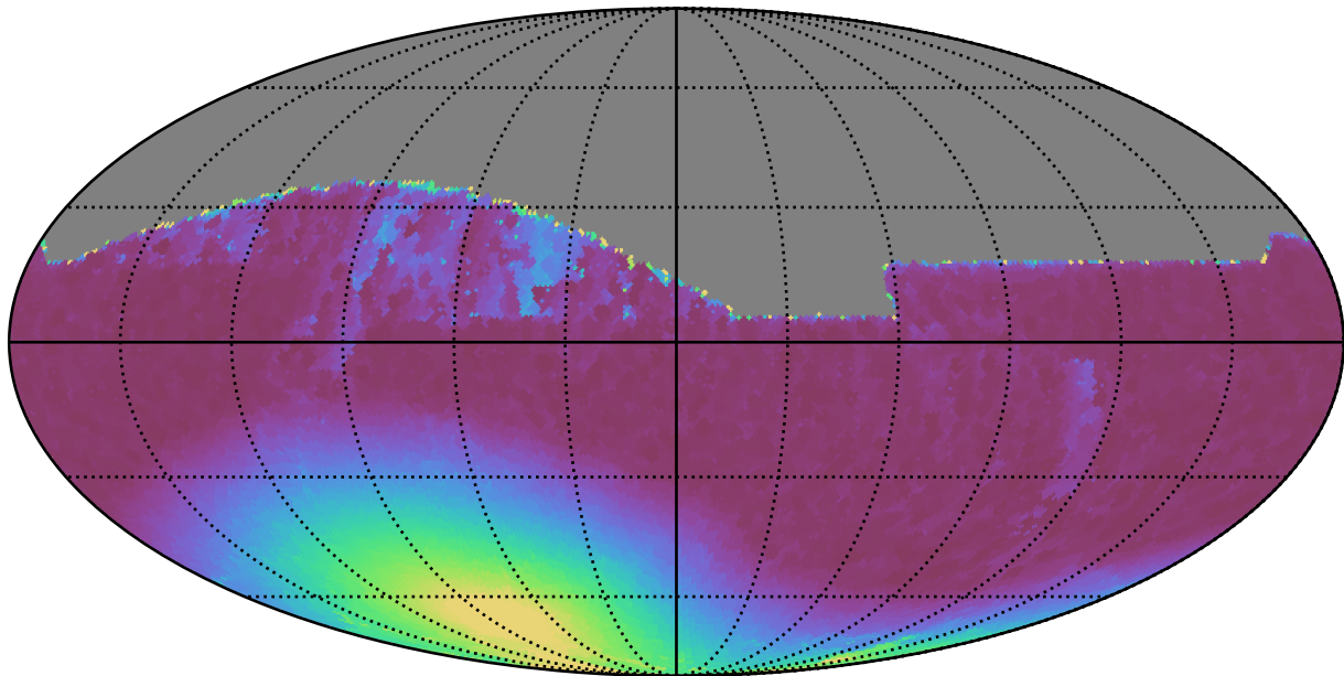
early_u_fpextra2.0_v3.4_10yrs All sky z band: Min moonDistance
