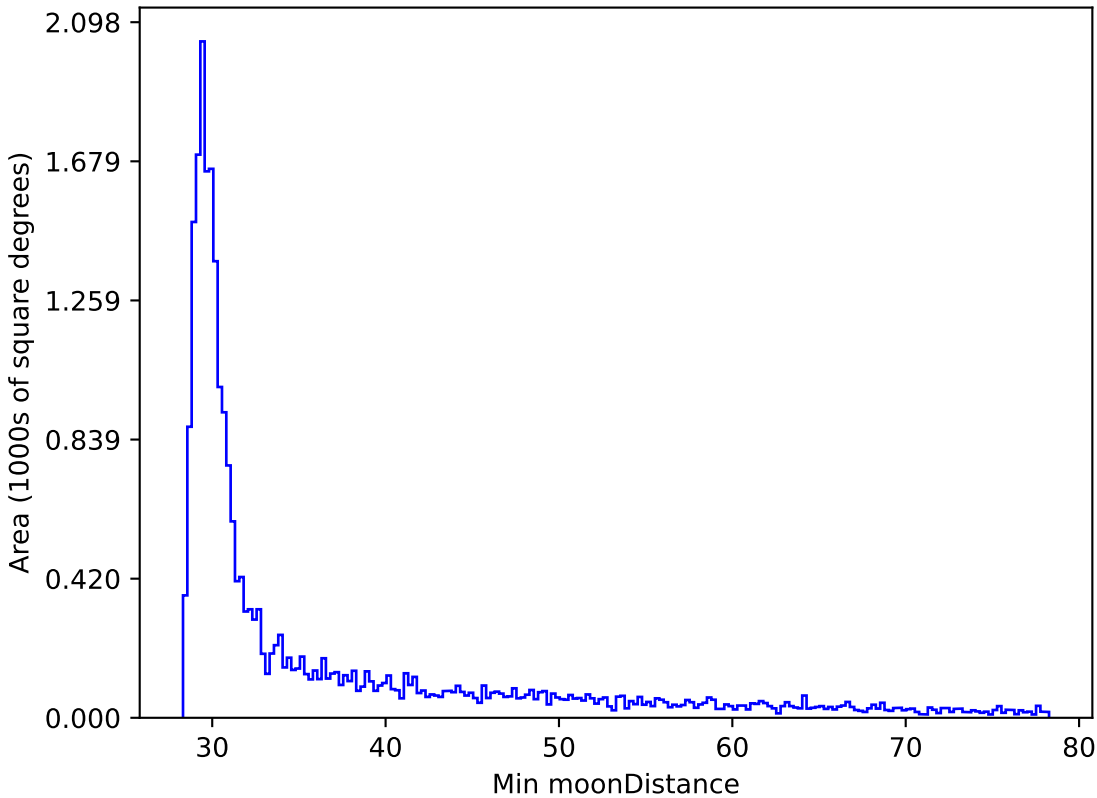
early_u_fpextra2.0_v3.4_10yrs All sky z band: Min moonDistance
