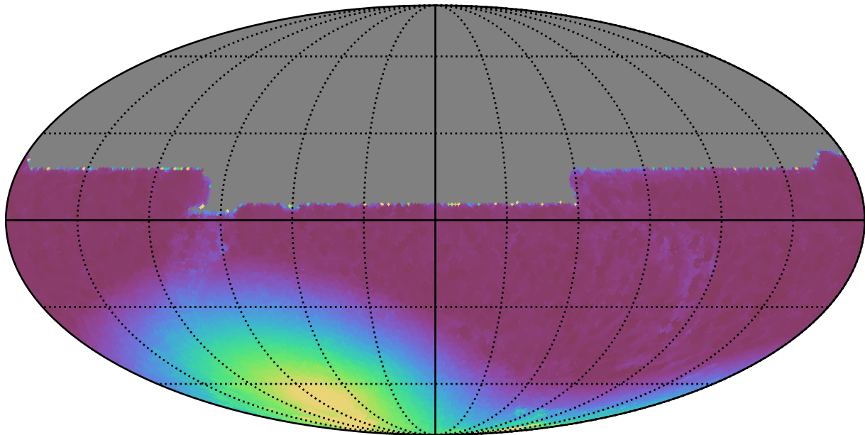
early_u_fpextra2.0_v3.4_10yrs All sky y band: Min moonDistance
