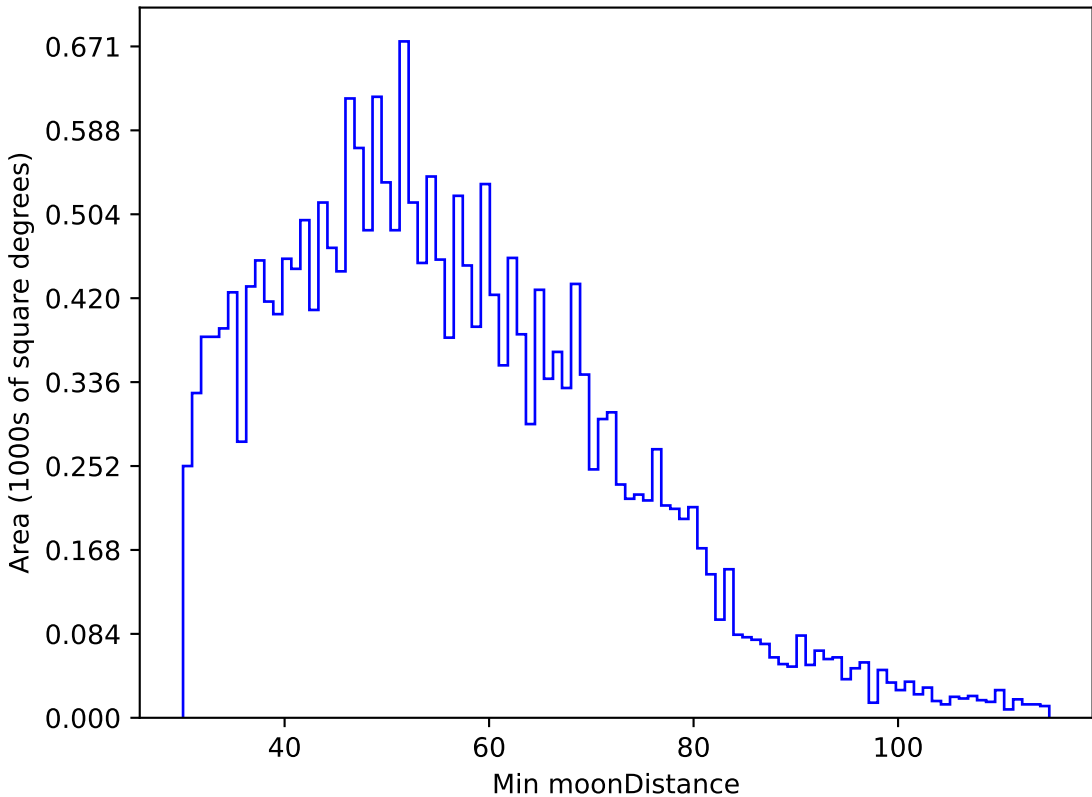
early_u_fpextra2.0_v3.4_10yrs All sky u band: Min moonDistance
