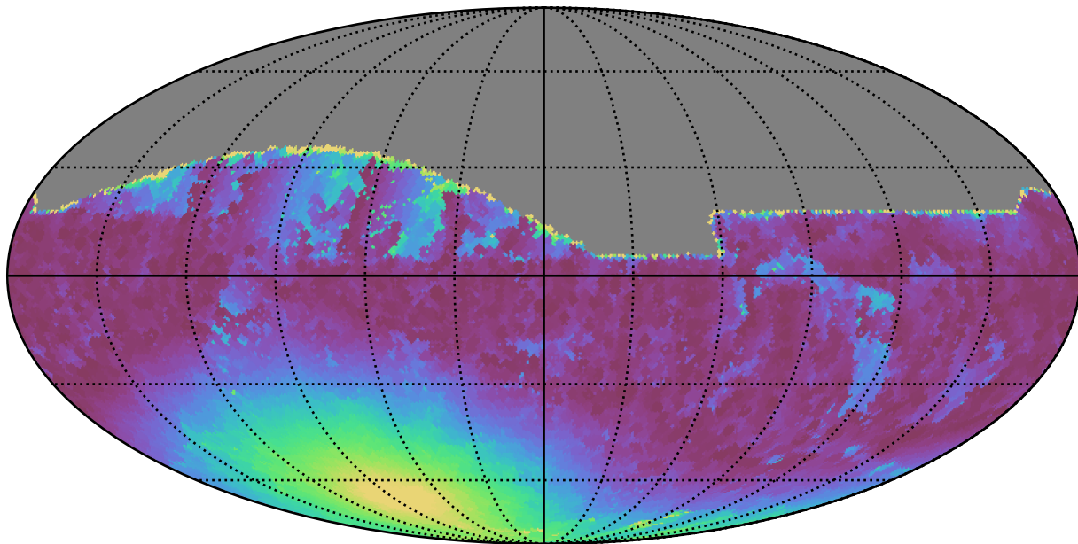
early_u_fpextra2.0_v3.4_10yrs All sky r band: Min moonDistance
