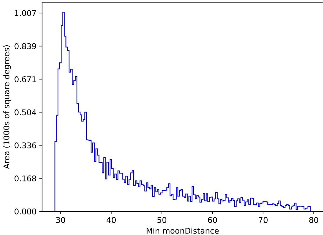
early_u_fpextra2.0_v3.4_10yrs All sky r band: Min moonDistance
