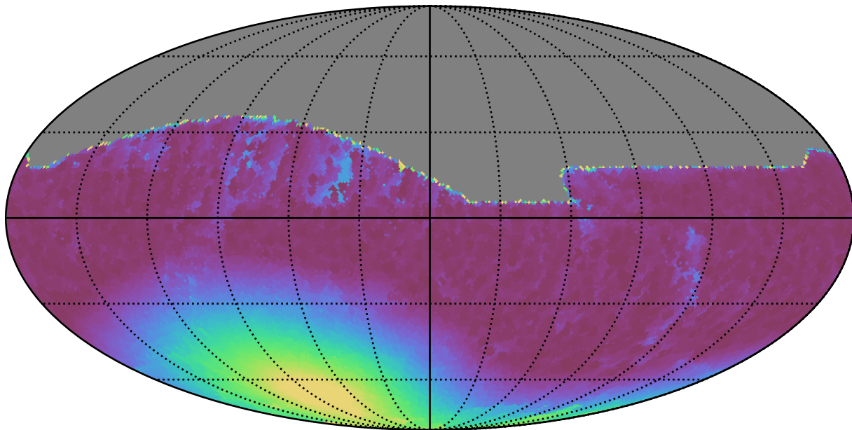
early_u_fpextra2.0_v3.4_10yrs All sky i band: Min moonDistance
