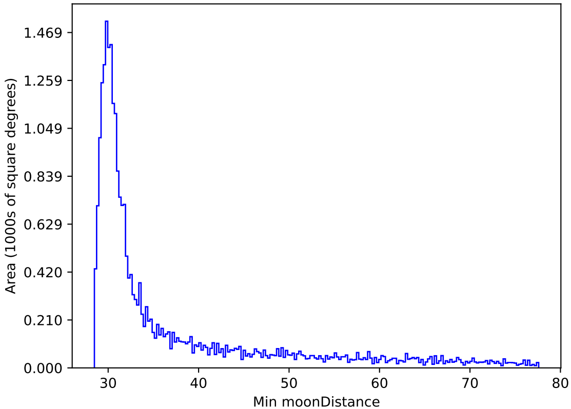
early_u_fpextra2.0_v3.4_10yrs All sky i band: Min moonDistance
