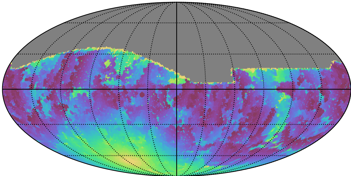
early_u_fpextra2.0_v3.4_10yrs All sky g band: Min moonDistance
