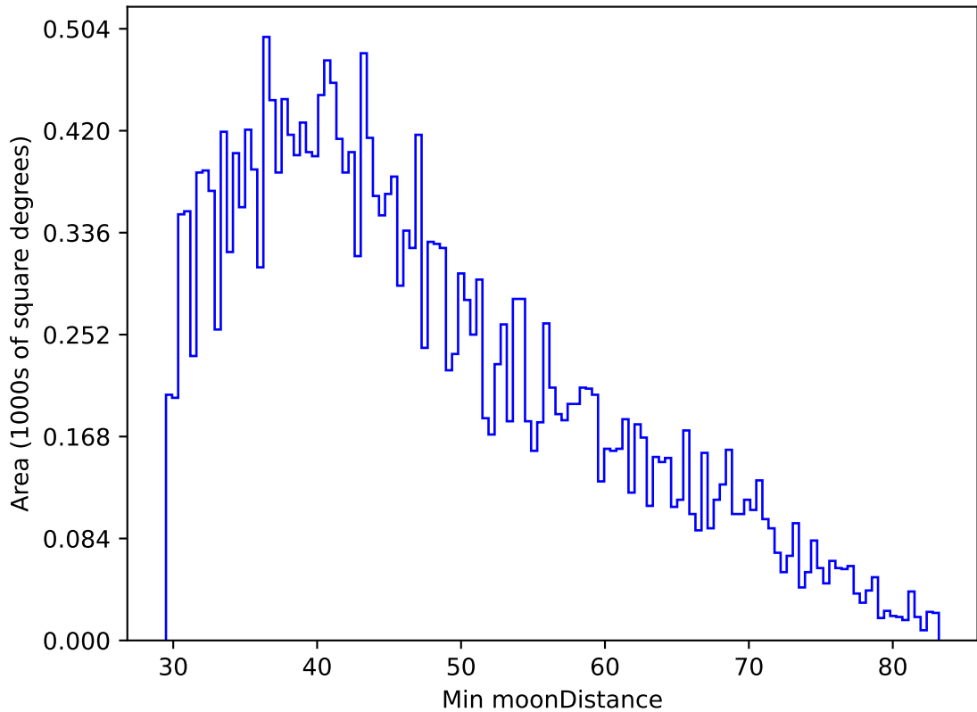
early_u_fpextra2.0_v3.4_10yrs All sky g band: Min moonDistance
