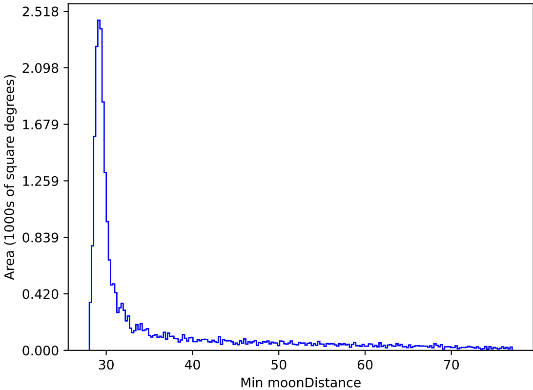
early_u_fpextra2.0_v3.4_10yrs All sky all bands: Min moonDistance
