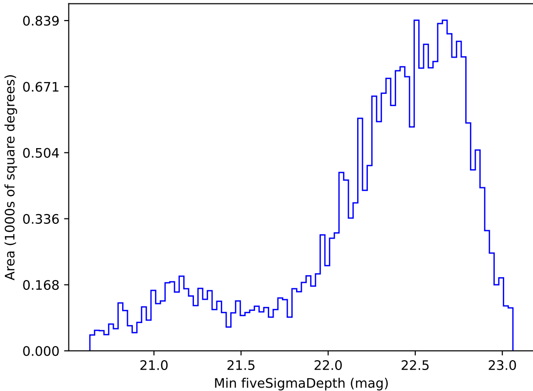
early_u_fpextra2.0_v3.4_10yrs Yr 1 z band: Min fiveSigmaDepth
