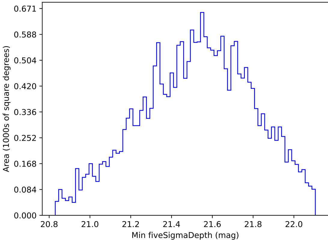
early_u_fpextra2.0_v3.4_10yrs Yr 1 y band: Min fiveSigmaDepth
