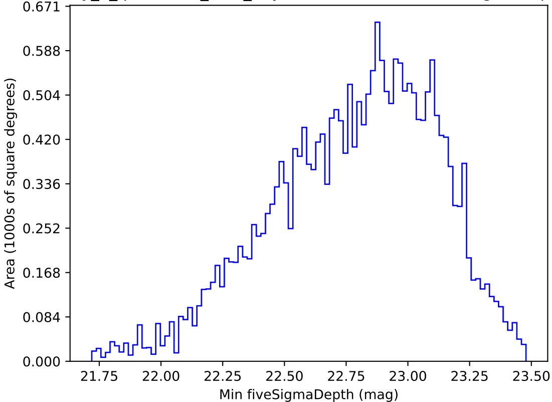
early_u_fpextra2.0_v3.4_10yrs Yr 1 u band: Min fiveSigmaDepth
