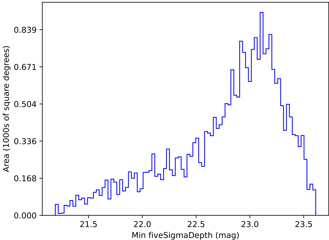
early_u_fpxextra2.0_v3.4_10yrs Yr 1 i band: Min fiveSigmaDepth
