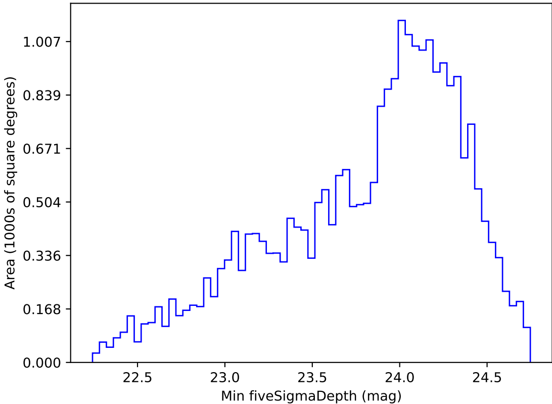
early_u_fpextra2.0_v3.4_10yrs Yr 1 g band: Min fiveSigmaDepth
