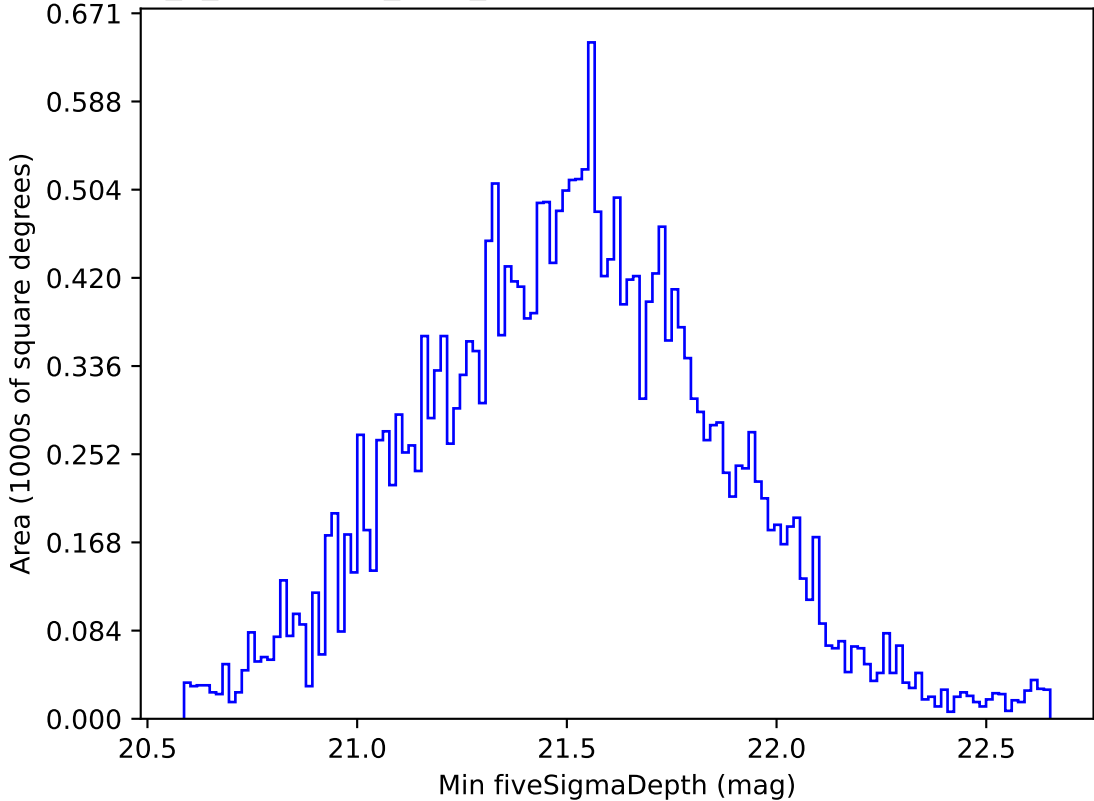
early_u_fpextra2.0_v3.4_10yrs Yr 1 all bands: Min fiveSigmaDepth
