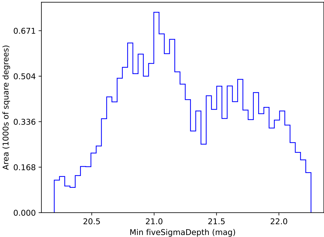
early_u_fpextra2.0_v3.4_10yrs WFD z band: Min fiveSigmaDepth
