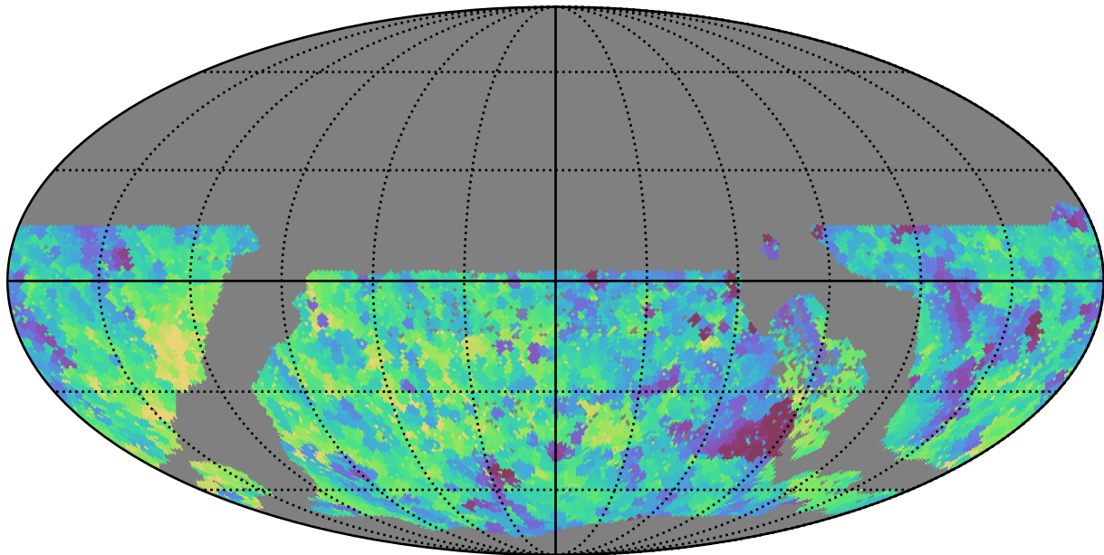
early_u_fpextra2.0_v3.4_10yrs WFD y band: Min fiveSigmaDepth
