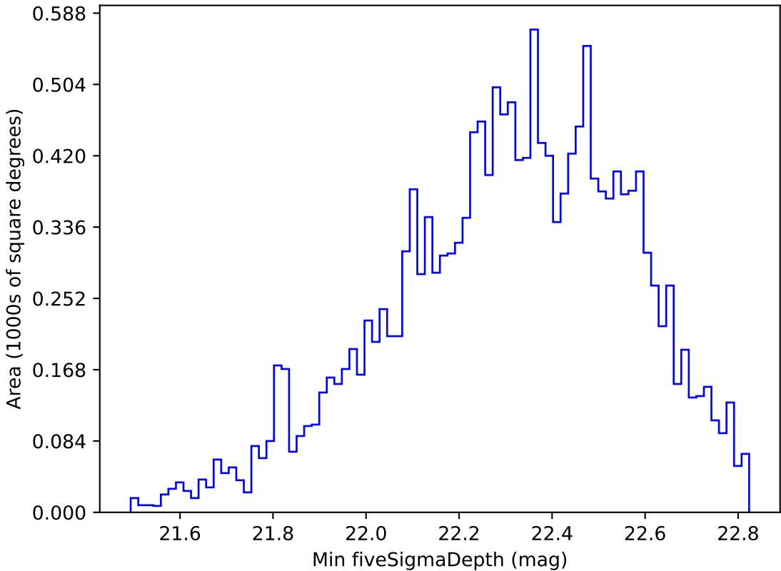
early_u_fpextra2.0_v3.4_10yrs WFD u band: Min fiveSigmaDepth
