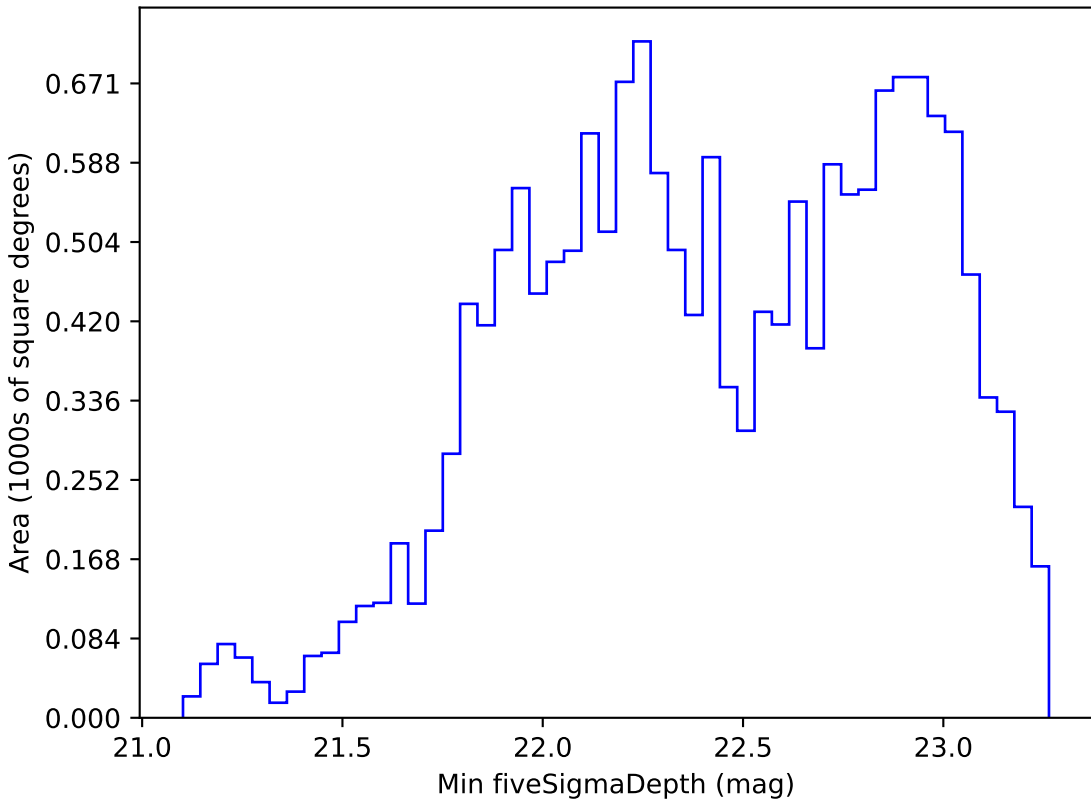
early_u_fpextra2.0_v3.4_10yrs WFD r band: Min fiveSigmaDepth
