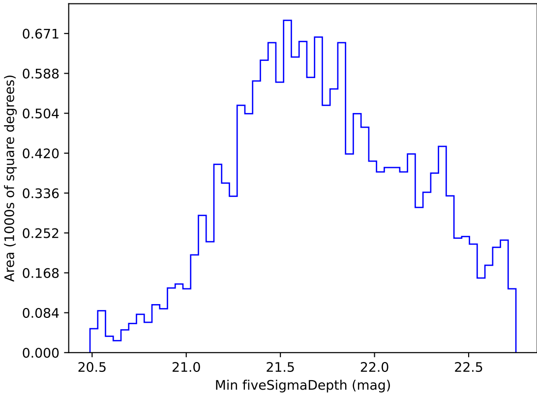
early_u_fpextra2.0_v3.4_10yrs WFD i band: Min fiveSigmaDepth
