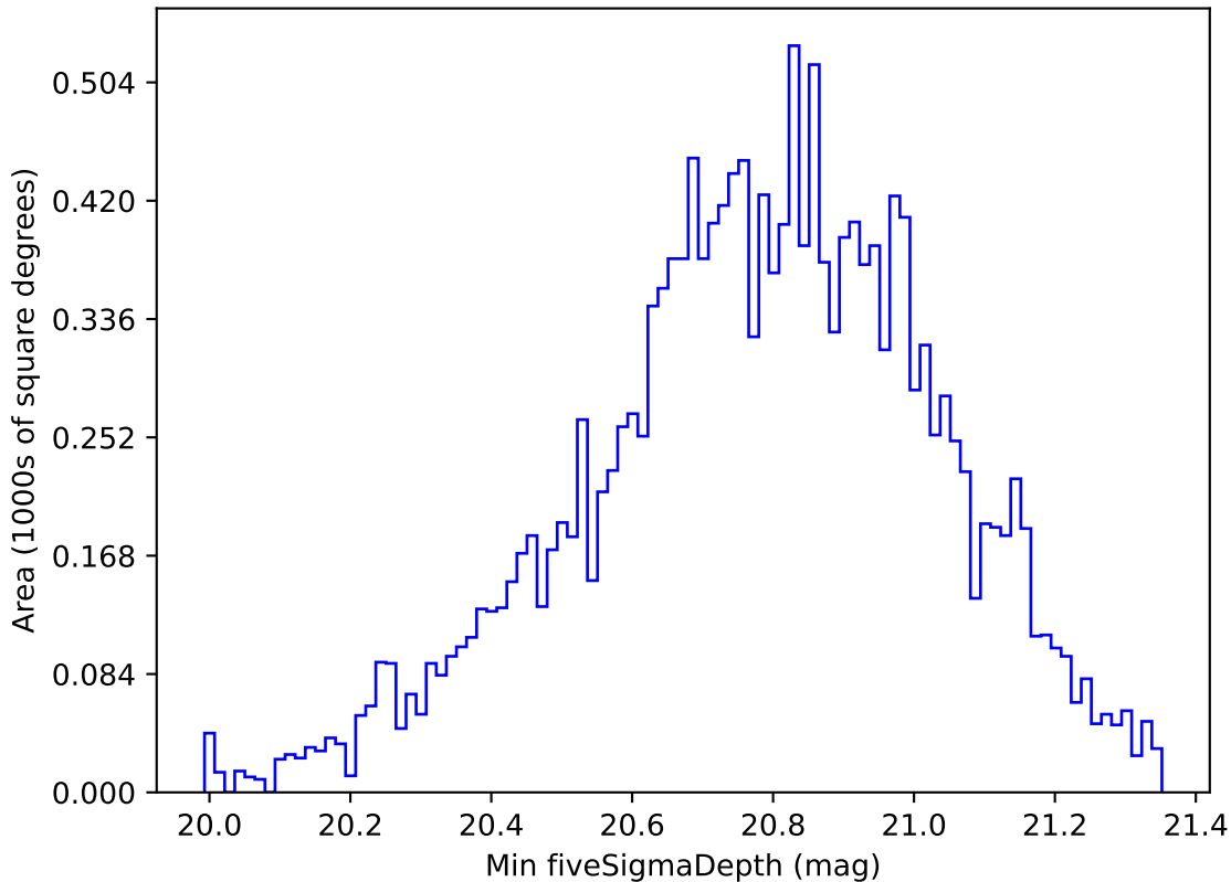
early_u_fpextra2.0_v3.4_10yrs WFD all bands: Min fiveSigmaDepth
