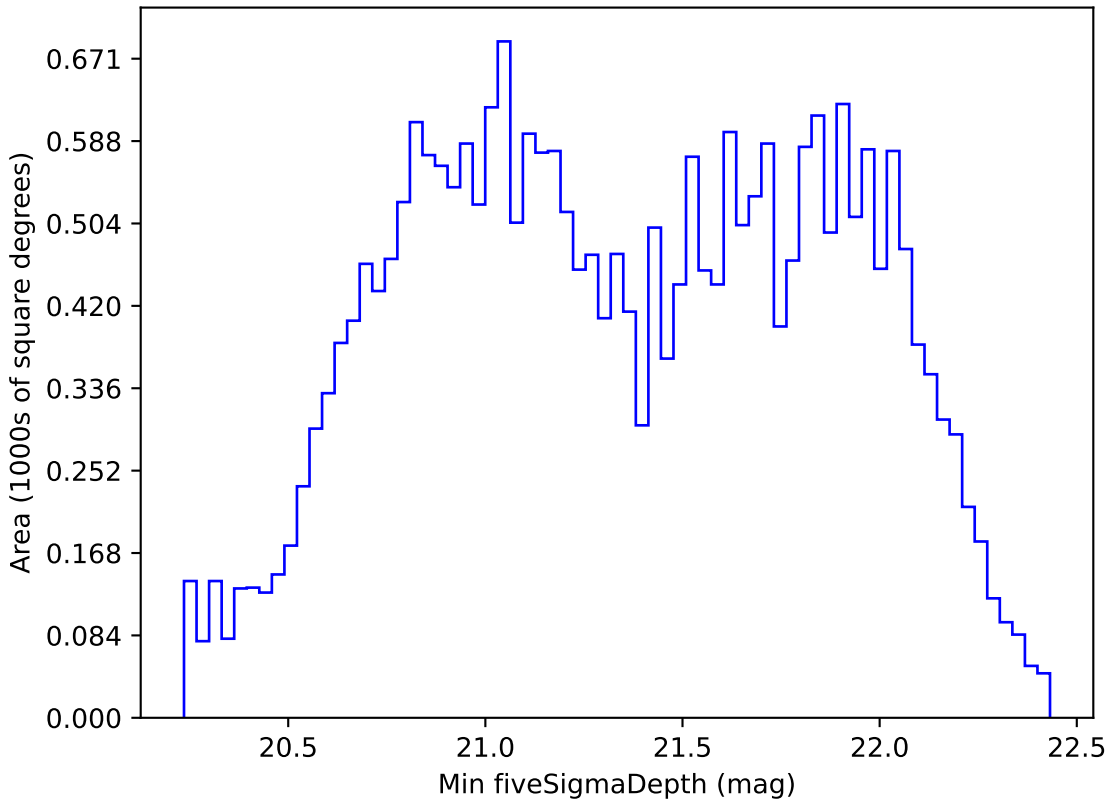
early_u_fpextra2.0_v3.4_10yrs All sky z band: Min fiveSigmaDepth
